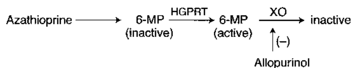
Figure VI-6-2. Drug Interaction Between Allopurinol and 6-Mercaptopurine
