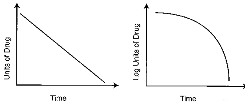
Figure I-1-9a. Plots of Zero-Order Kinetics
