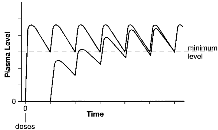
Figure I-1-13. Effect of a Loading Dose on the Time Required to Achieve the Minimal Effective Plasma Concentration
